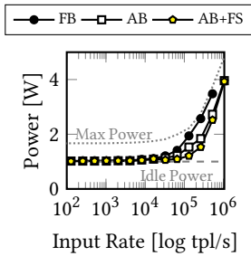
Figure 4: Adaptive batching and frequency scaling.
